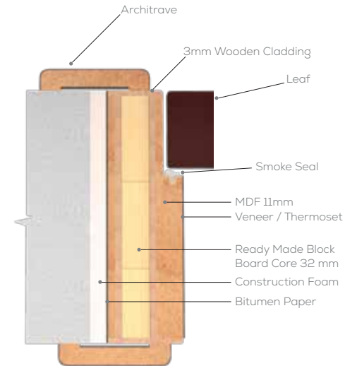
VENEERED JAMB FRAME (VENEERED, THERMOSET & PAINTED)
